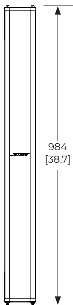
Vista frontal
